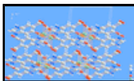
Fig. 2. A view of the three-dimensional structure of the title compound along the b axis. Hydrogen bonds are shown as dashed lines.
